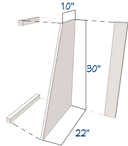
OSB LEG DETAIL
